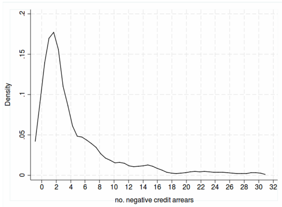
Figure 4 Kernel Density graph Number of credit arrears before the first credit arrear removal.
