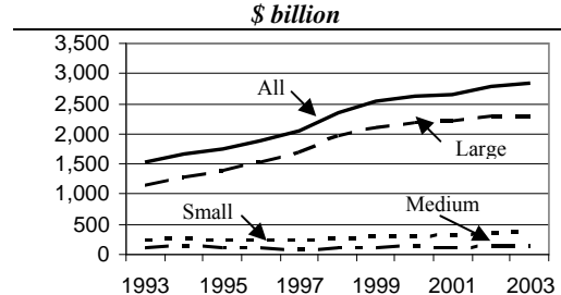
Liquidity creation 1993 - 2003
